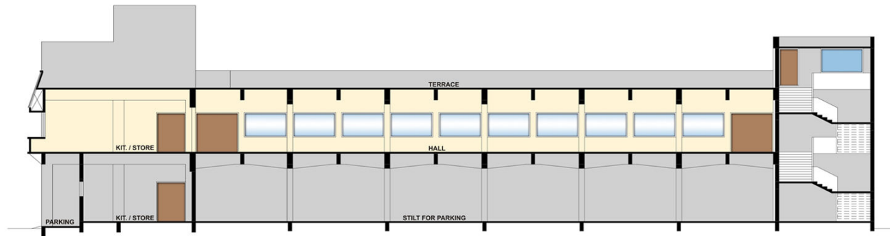
SECTION 4 - 4
