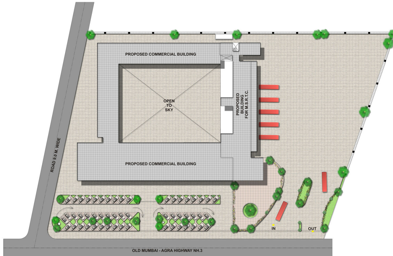
PROPOSED SITE PLAN OF DEOPUR BUS STAND
