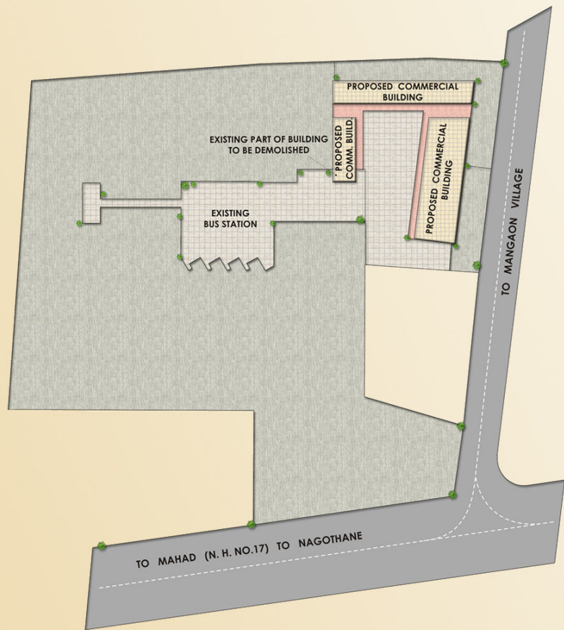
SITE PLAN
