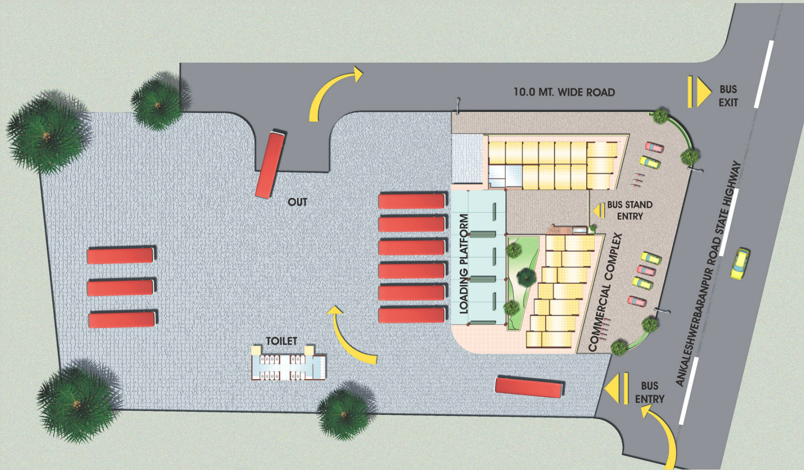
SITE PLAN
